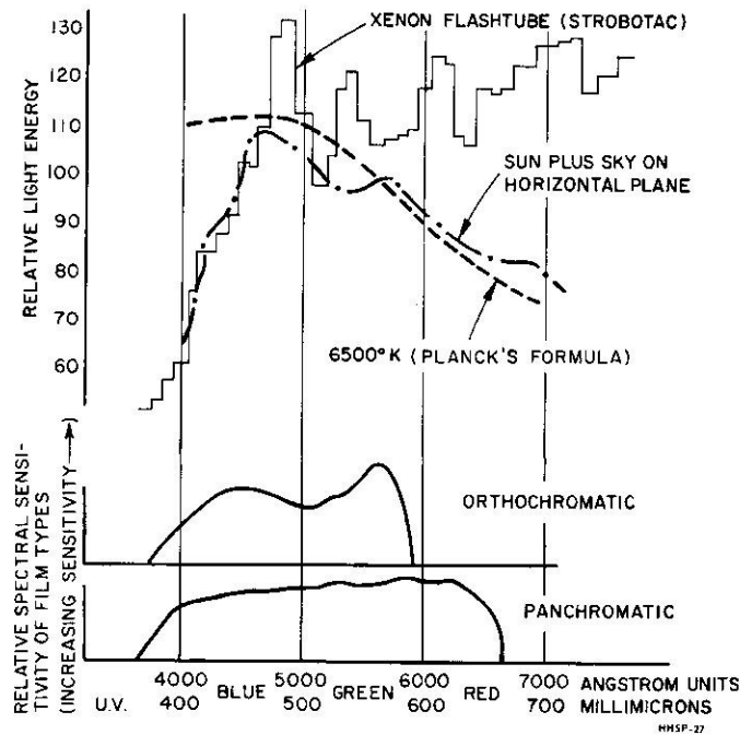
Figure 5-6. Spectral distribution of light output from GenRad stroboscopes.
