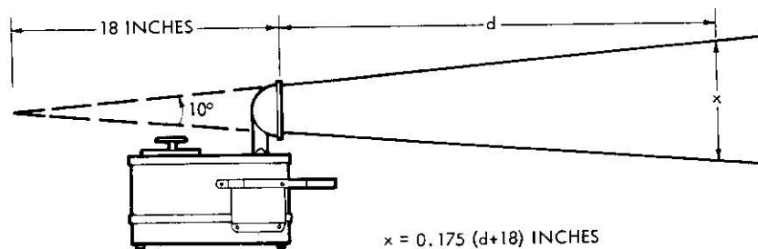
Figure 5-5. Beam width characteristics of Strobotac and Stroboslave with reflector in place.
