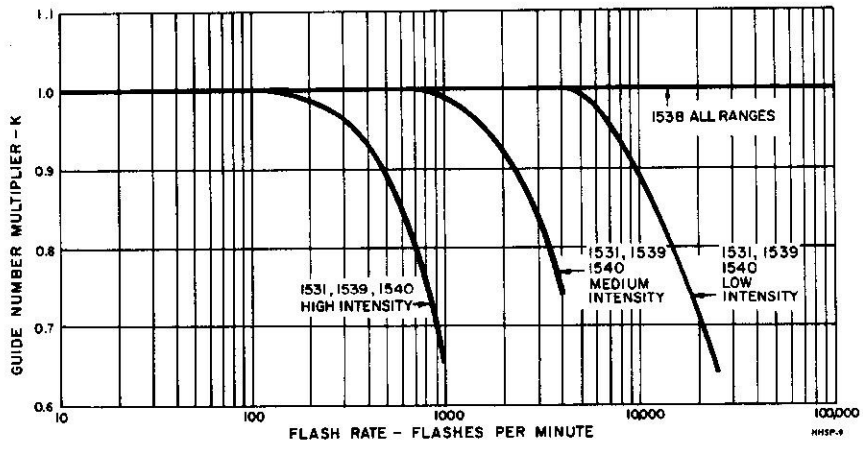
Figure 5-9. Guide-number correction for repetitive flashing.
