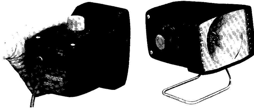
Figure 2-7. GR 1543 Stroboscope, an inexpensive yet complete and versatile stroboscope. It can be hand held (left) or mounted on stand supplied (right). The 1544 is nearly identical in appearance, while the 1542 is similar in shape but slightly smaller.
