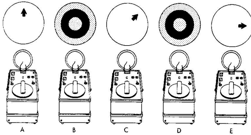
Figure 1-1. How the stroboscope produces a slow-motion image. The stroboscope above is flashing once every 1 \frac{1}{8} revolution of the disk. In A, a single flash catches the disk in its 0^\circ position. In B, while the stroboscope is not flashing, the disk, rotating clockwise, makes better than a full revolution. In C, the next flash catches the disk at its 45^\circ position. The next flash, in E, occurs after the stroboscope has made another 1 \frac{1}{8} revolution. The eye, retaining each image it receives for a split second, weaves A, C, and E into an image of apparent slow forward motion.
