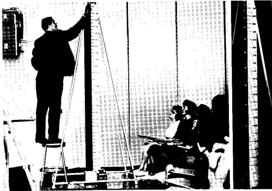
Figure 6-1. Ball is dropped alongside calibrated scale while camera takes multiple-image photo by light of Strobotac (at bottom of scale). Resulting photo (right) is proof of acceleration.
