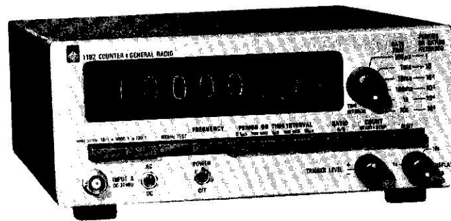
Figure 3-6. Counters can be used for precision speed measurements. The 1192 is typical of the low-cost universal counters available today. These counters can be used with appropriate transducers, such as photoelectric pickoffs, for speed measurements. They also can be connected to the output of a stroboscope to act as either a calibrator or monitor, where precise measurements are required. Counters read directly in terms of frequency, i.e., events per second. Hence, the reading must be multiplied by 60 to get rpm.
