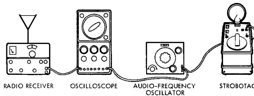
Figure 6-30. Flashing rate can be calibrated in terms of standard frequencies generated locally or received off the air.
