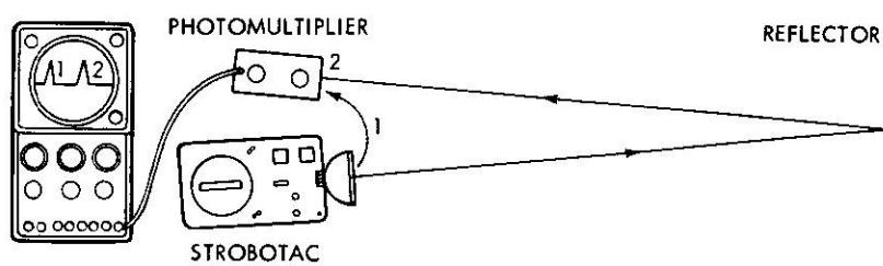
Figure 6-2. Light reaching photomultiplier directly from Strobotac and reflected from wall causes two distinct pulses on oscilloscope, proving finite velocity of light.
