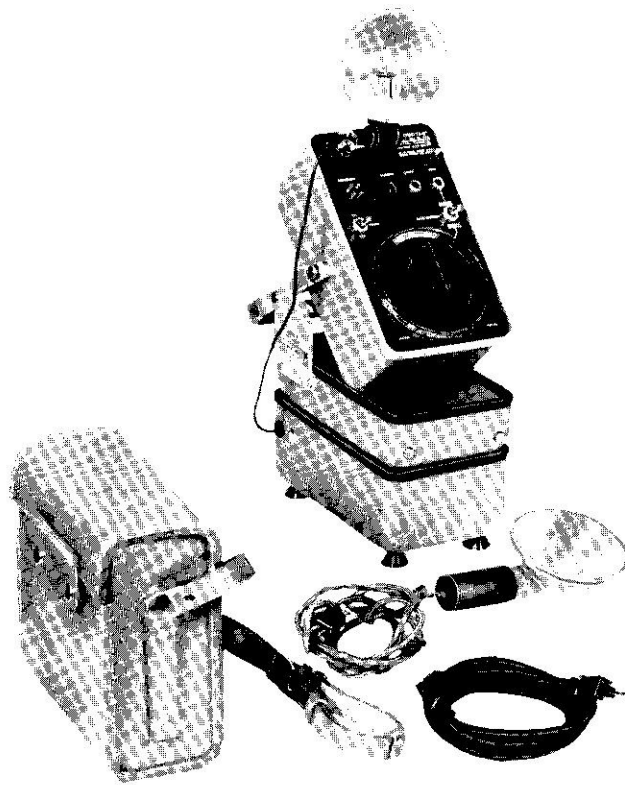
Figure 2-3. GR 1538-A Strobotac electronic stroboscope with accessories. Left foreground, in leather case, are battery and charger. Power cable is in right foreground, and extension lamp is next to Strobotac, which sits atop plug-in high-intensity-flash capacitor.
