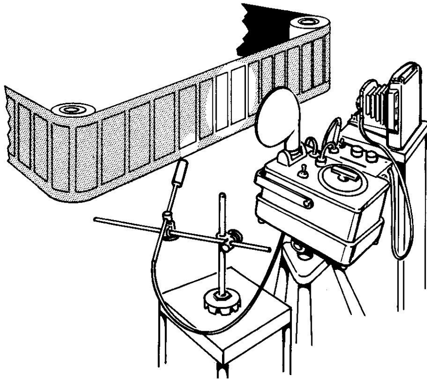
Figure 5-3. With flash delay set to MULT and Strobotac photoelectrically synchronized with roll labels, photographer adjusts delay for desired picture. He then switches flash delay to SINGLE FLASH, after which the tripping of the camera shutter will cause one flash to be generated at the right moment for the picture.
